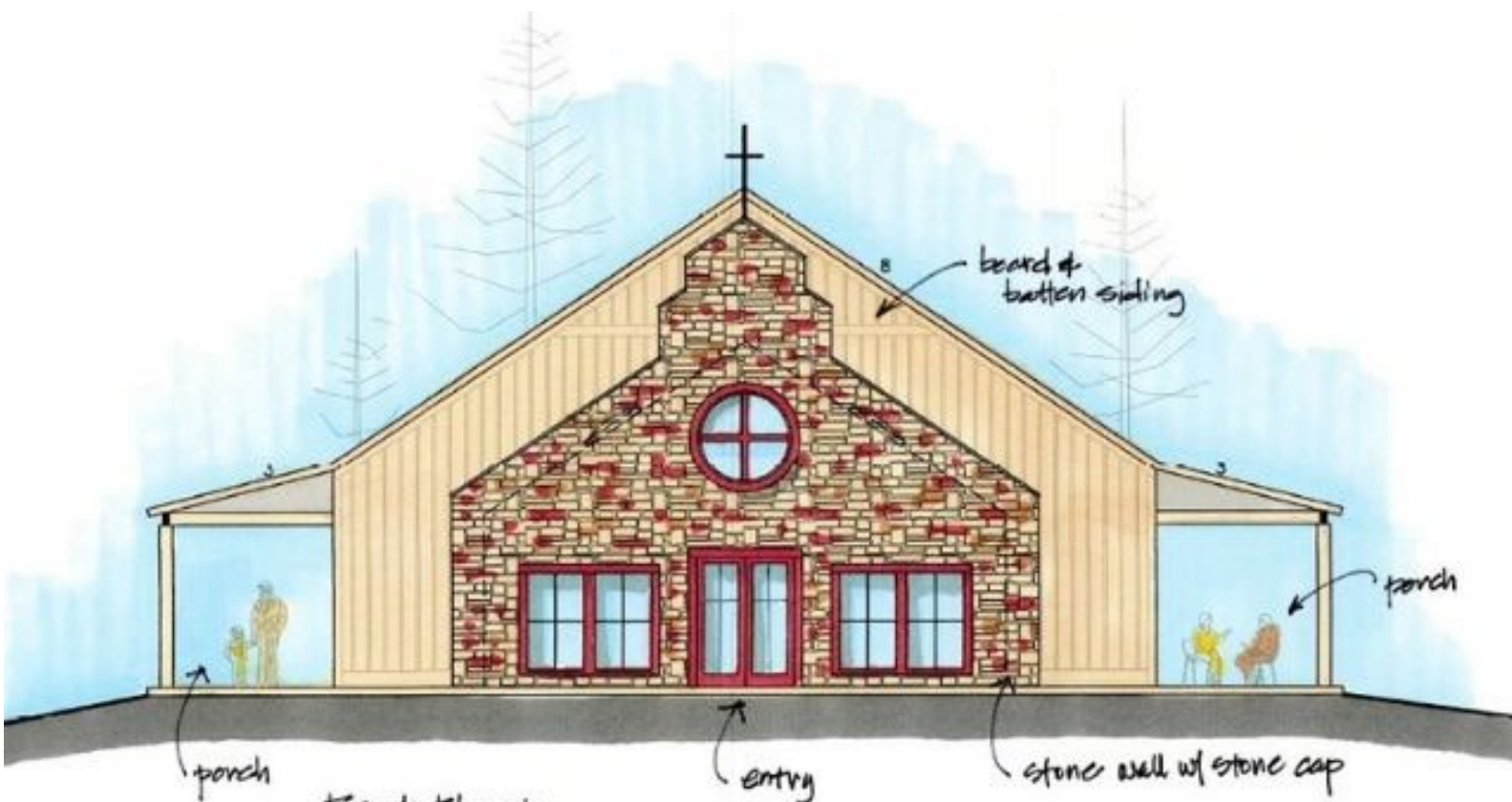
Front Elevation scale 1/8" = 1'-0"
